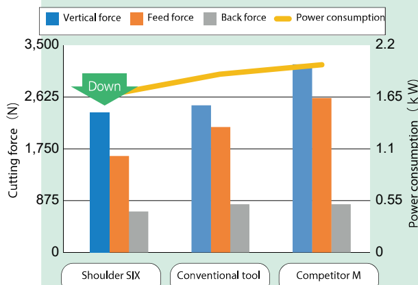
Small a_p cutting condition ( a_p=3\text{mm} , a_e=40\text{mm} )
