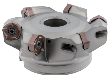
Coarse Pitch ( \varnothing 100\text{mm} / 6 flutes)
